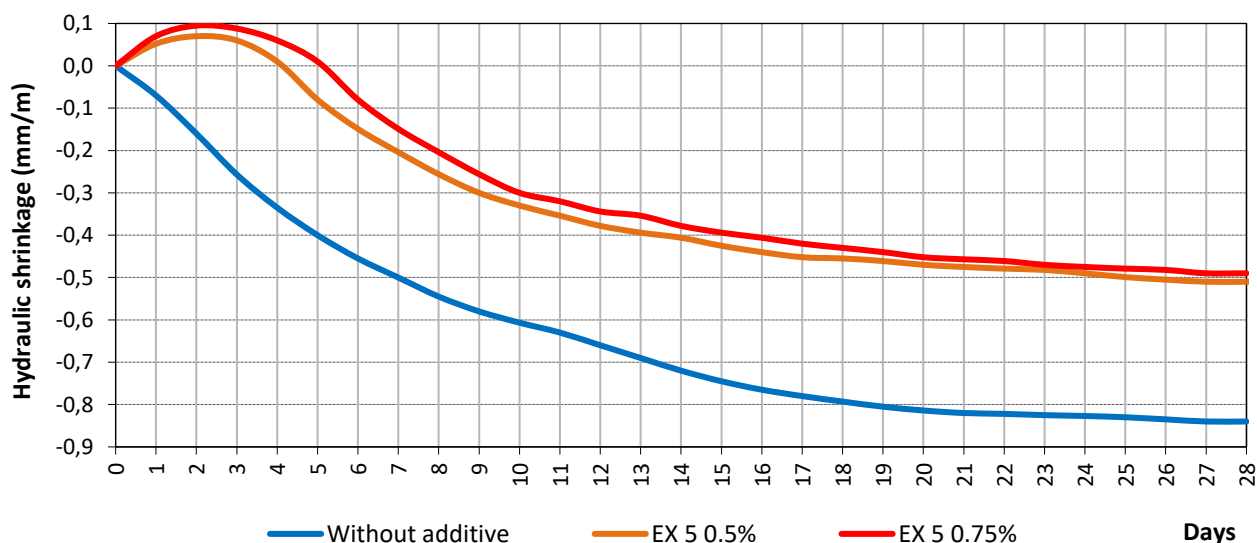
Trends of shrinkages at different dosages on a standard mortar of Pentachem
